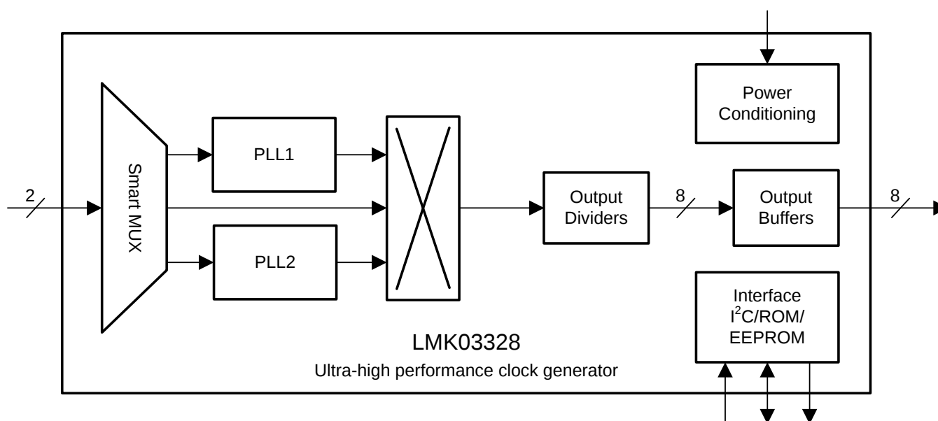
LMK03328 Simplified Block Diagram
